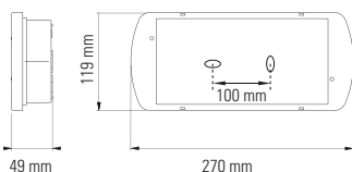
UNILED 2-8 / 2-8 ES (mm)
